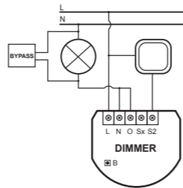
Fig.3 Wiring diagram for connecting the Bypass
